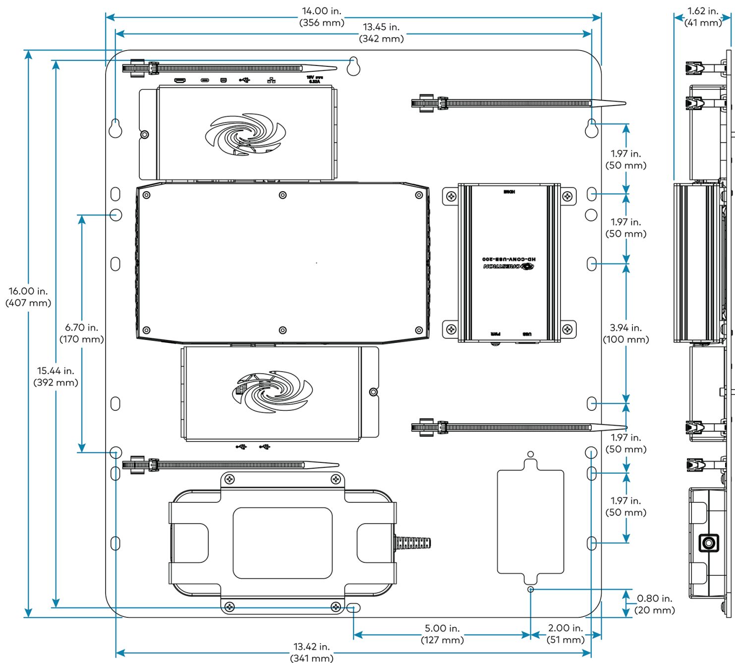
UC-BRKT-100-ASSY
